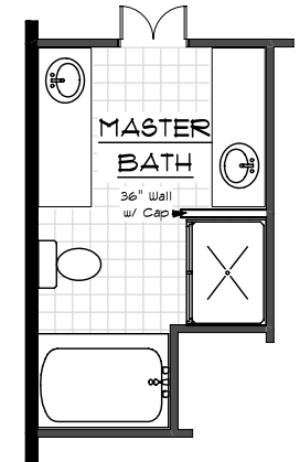
Garden Bath with 4' Shower Option
